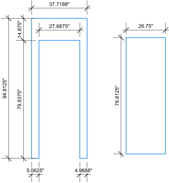
A2 Sintra Door Cladding Image/Live Area 37.7188" x 94.8125"H
